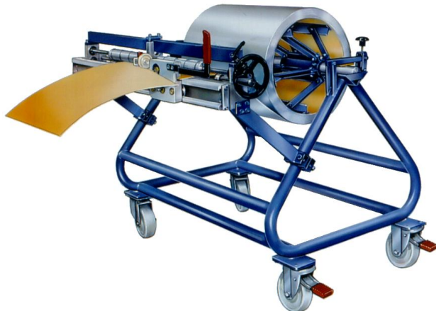
Decoiler K1-CW/AQ
